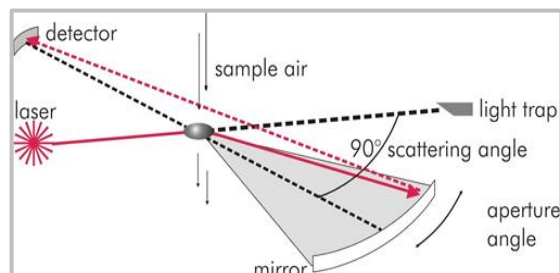
Measurement principle
